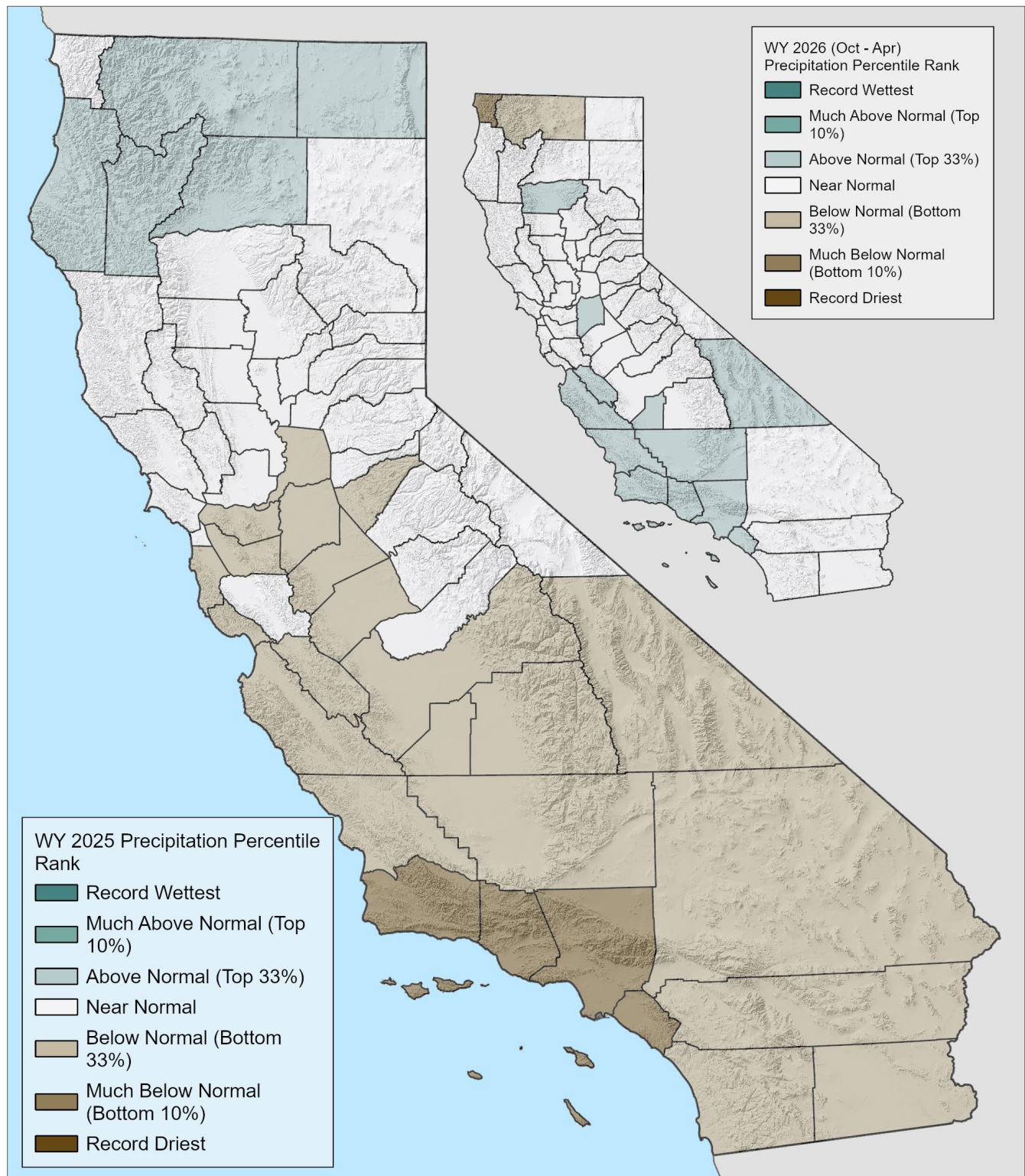
Figure 3: Precipitation Percentiles - 2025 and 2026 Water Year Precipitation NOAA National Centers for Environmental Information ( Climate at a Glance: Precipitation )
