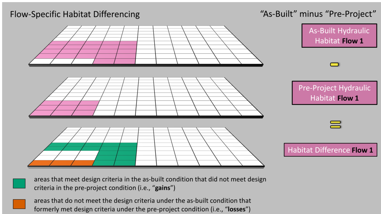
Figure 3. Example showing the differencing of the "as-built" and "pre-project" DEMs at a single flow in the range of design flows to identify the flow-specific areas of habitat gains (i.e., spatially explicit areas that meet design criteria in the as-built condition that did not meet design criteria in the pre-project condition; green cells) and habitat losses (i.e., spatially explicit areas that do not meet the design criteria under the as-built condition that formerly met design criteria under the pre-project condition; red cells).
