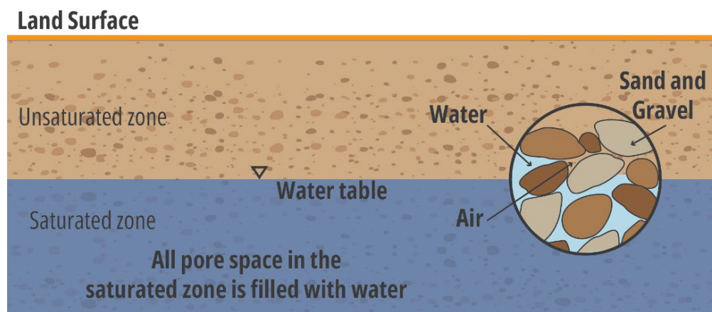
Figure 2: Pore space is filled with air and water in the unsaturated zone and with water in the saturated zone.
